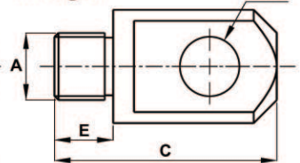
Plunger
