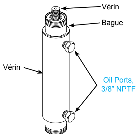
Figure 1 - Composants de vérin type
