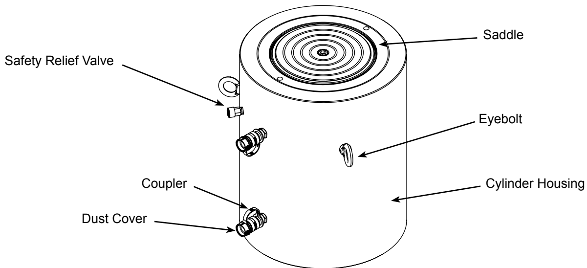
Figure 1 - Typical Double-Acting Cylinder Components
