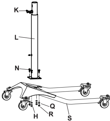
Figure 3 - Attaching Column to Base Frame
