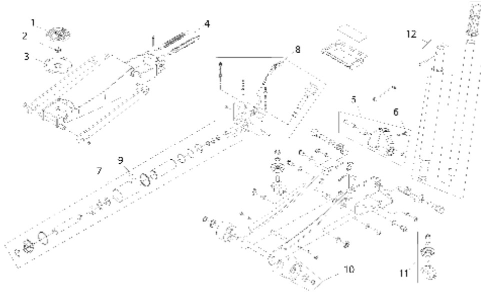
Figure 4 - Replacement Parts Illustration for Model 29028.
